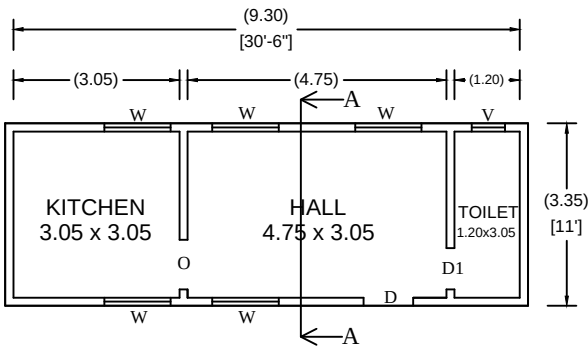
PROP. GROUND FLOOR PLAN
