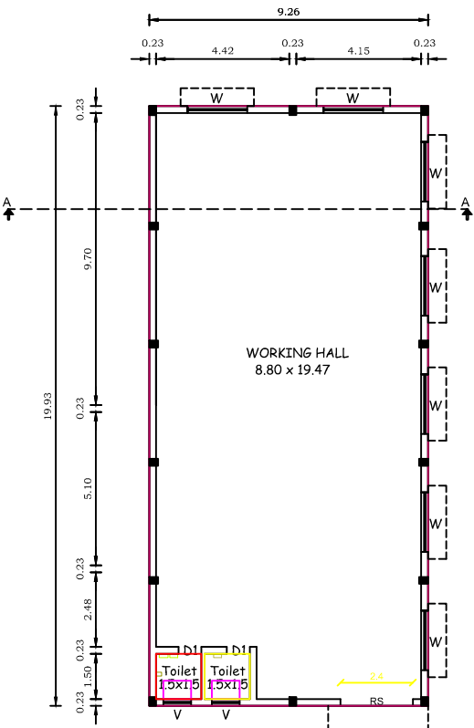
PLAN
