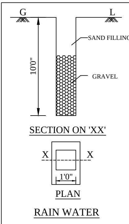
RAINWATER HARVESTING
