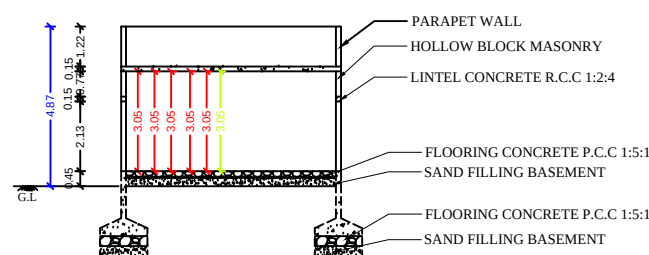
SECTION ON'AA'
