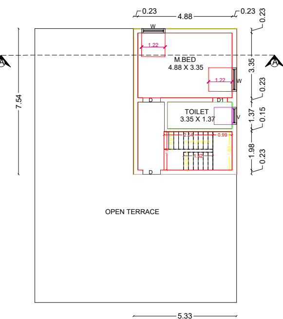
PRO.FIRST FLOOR (F.F) PLAN
