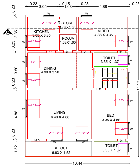
PRO.GROUND FLOOR (G.F) PLAN
