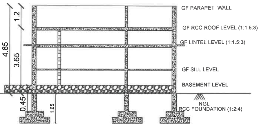
SECTIONAL VIEW ON A-A
