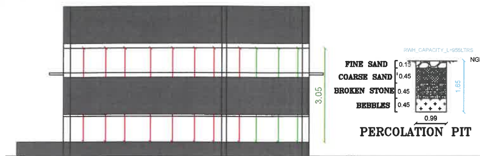
SOUTH ELEVATION
