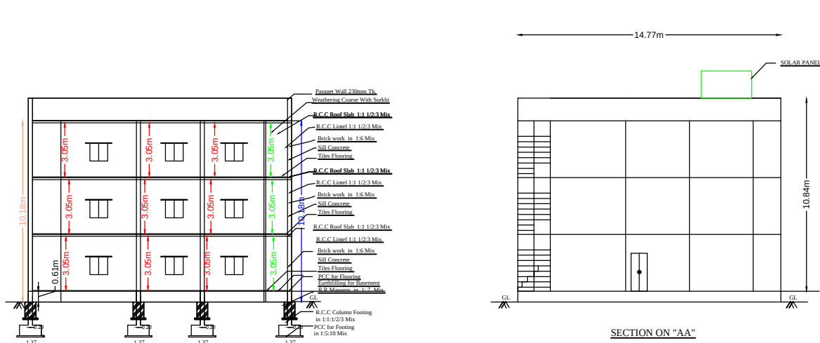
SIDE ELEVATION
