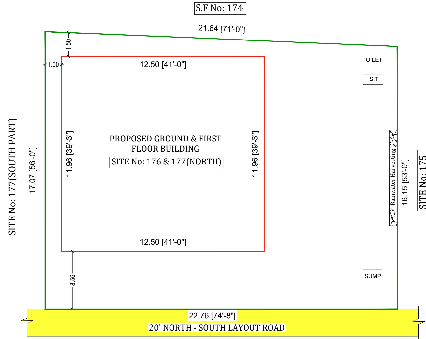
SITE PLAN
