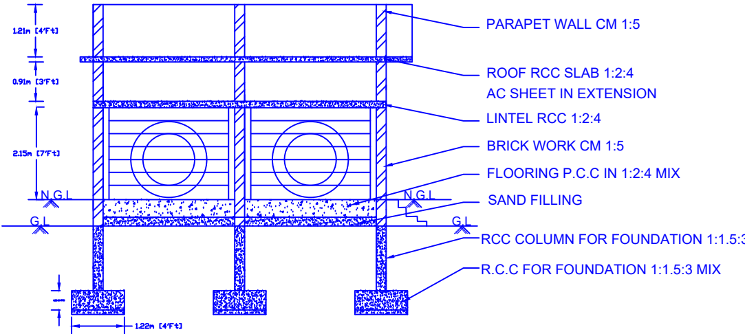
SECTION ON-AA
