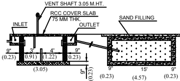
SECTION ON SEPTIC TANK & DISP-TRENCH
