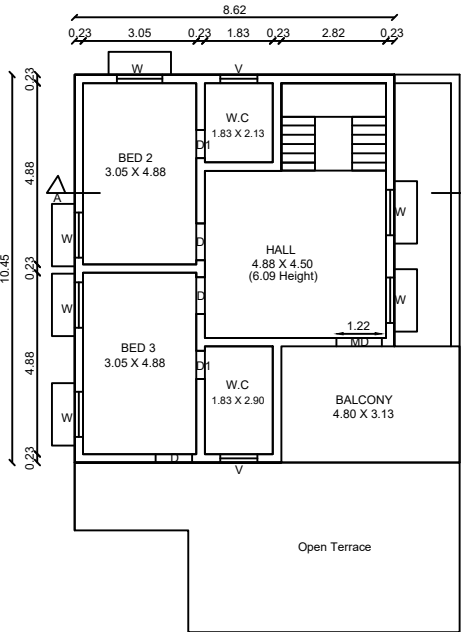
PROPOSED ADDITIONAL FIRST FLOOR PLAN
