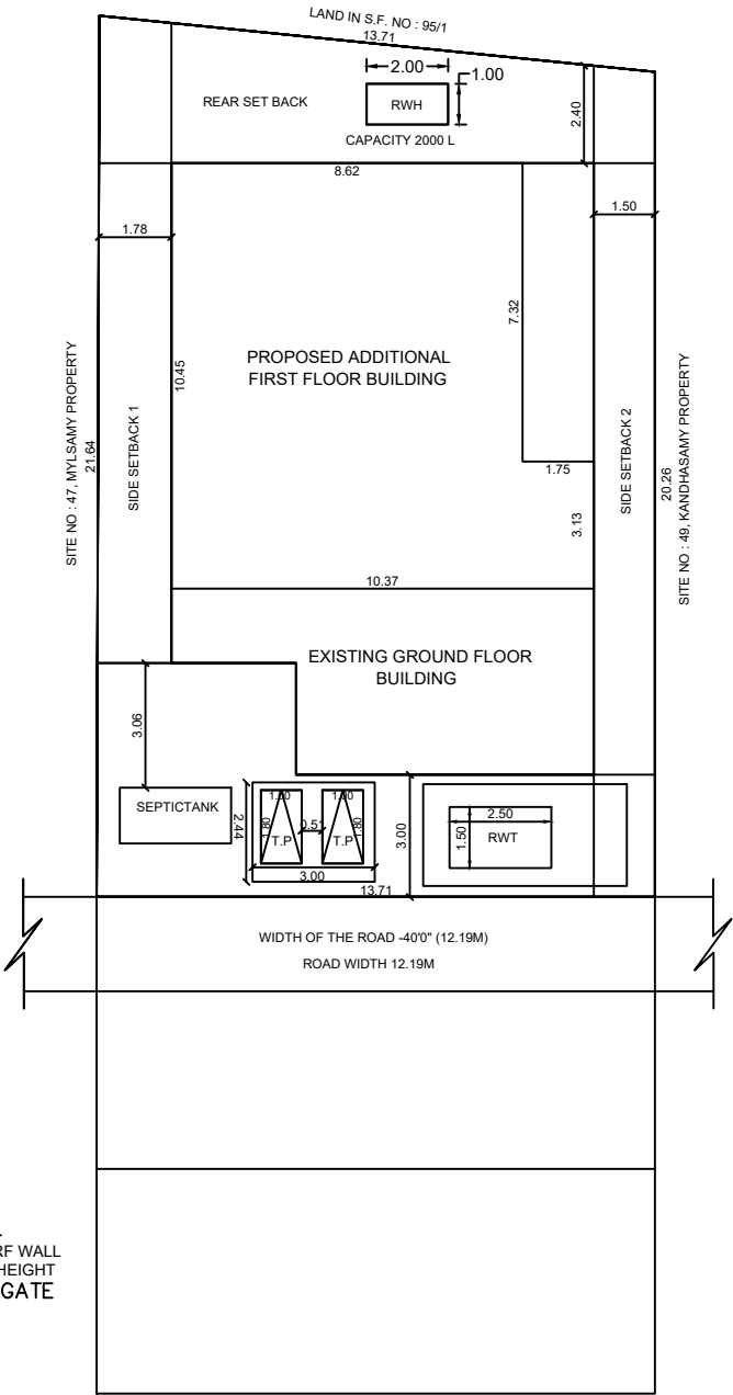
SITE PLAN
