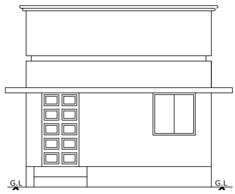
ELEVATION FACING NORTH
