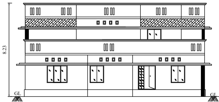
FRONT ELEVATION (FACING EAST)
