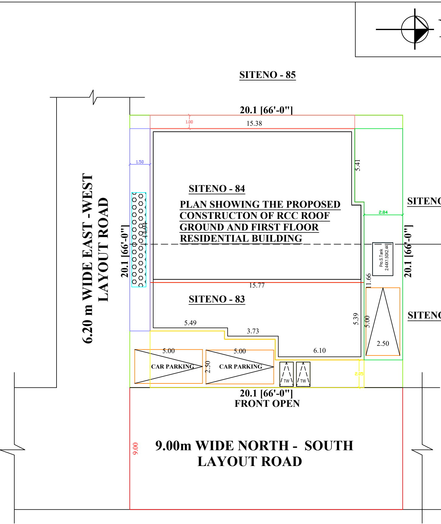
SITE PLAN AND TERRACE PLAN
