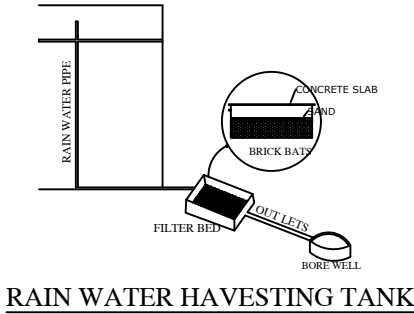
RAIN WATER HAVESTING TANK
