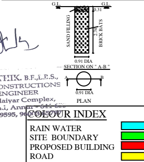
DETAILED PLAN OF RAINWATER PERCULATION&COLLECTION PIT
