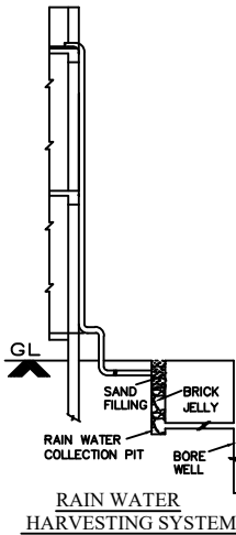
RAIN WATER HARVESTING SYSTEM
