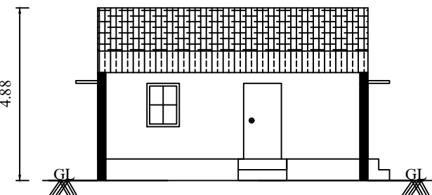
ELEVATION (FACING EAST)
