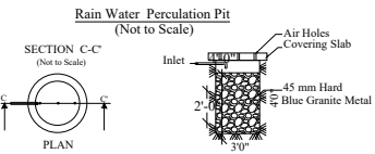
RAIN WATER PERCOLATION PIT (Not to Scale)
