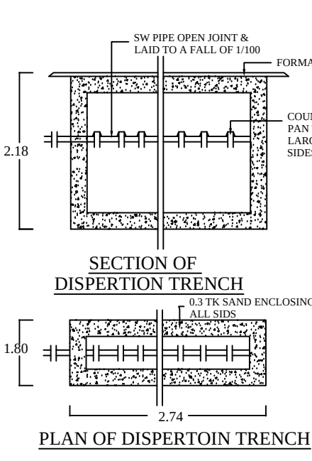
DISPERSION TRENCH
