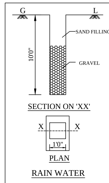
RAINWATER HARVESTING
