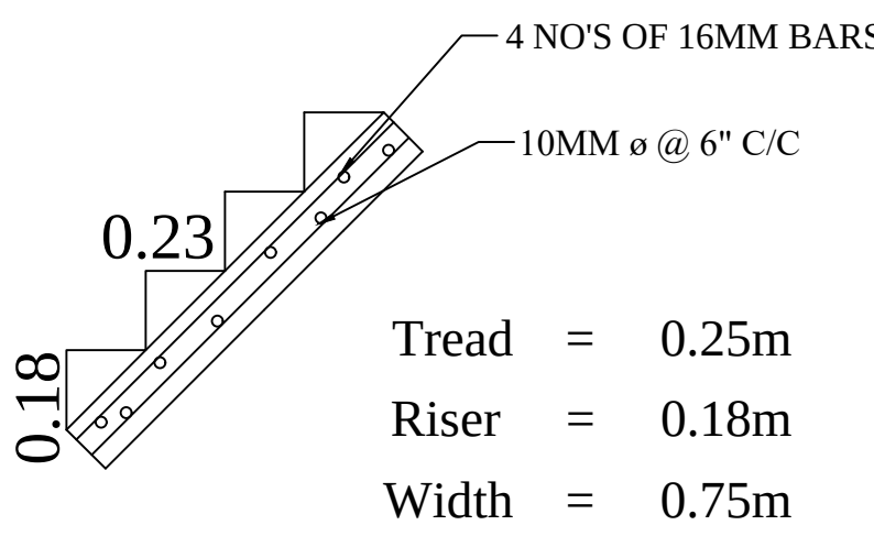
STAIRCASE DETAILS
