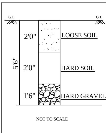
TRIAL PIT
