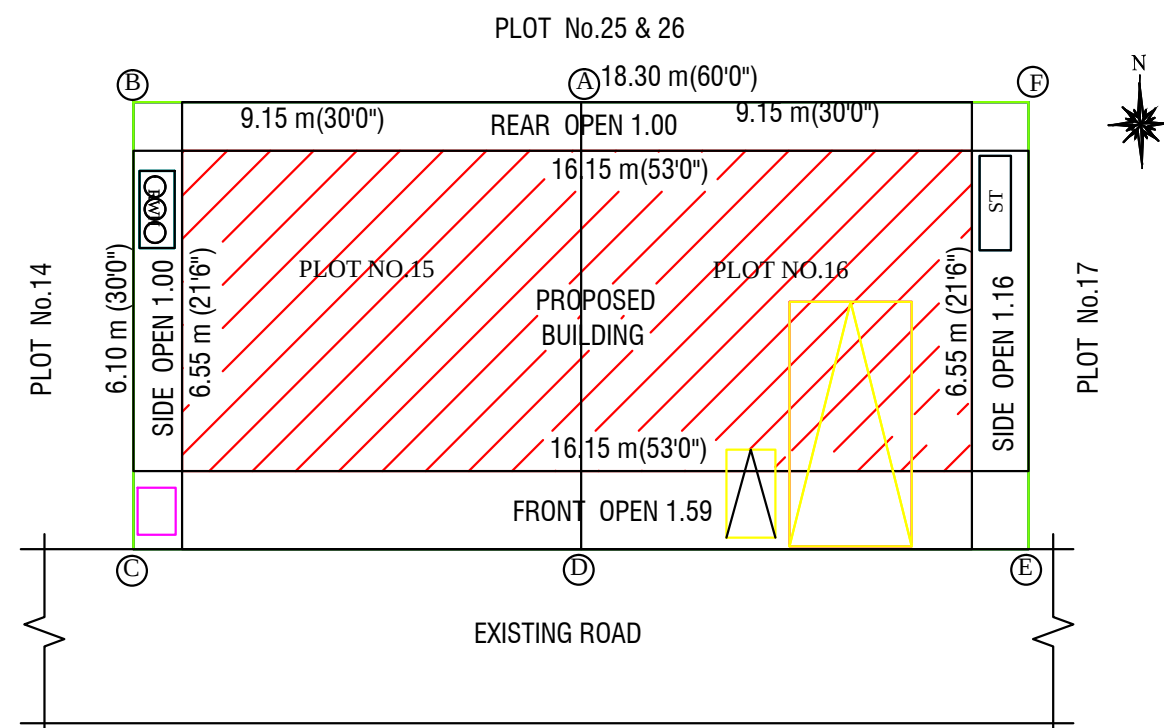
SITE PLAN
