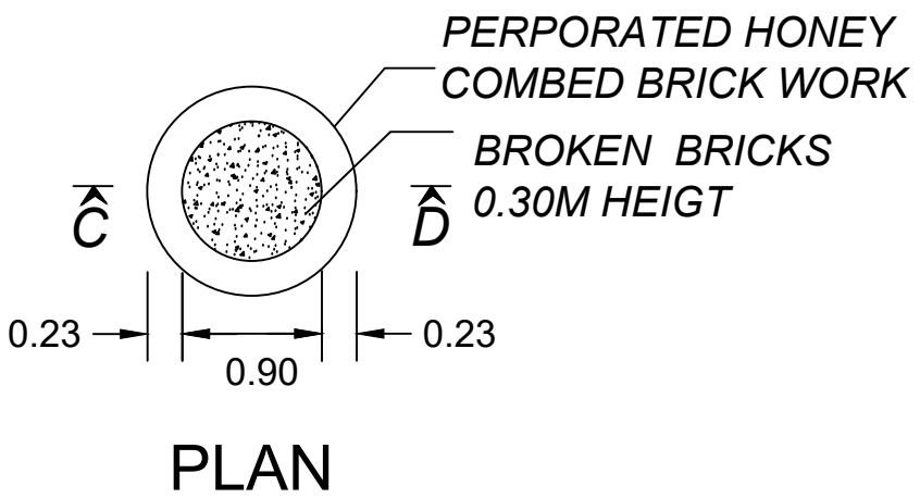
RAIN WATER HARVESTING BY PERCOLATION RECHARGE PIT METHOD
