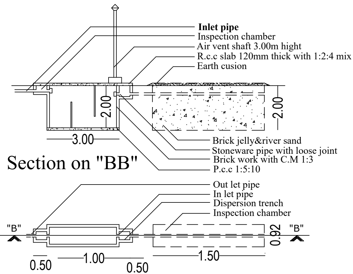
Plan of septic tank and dispersion trench
