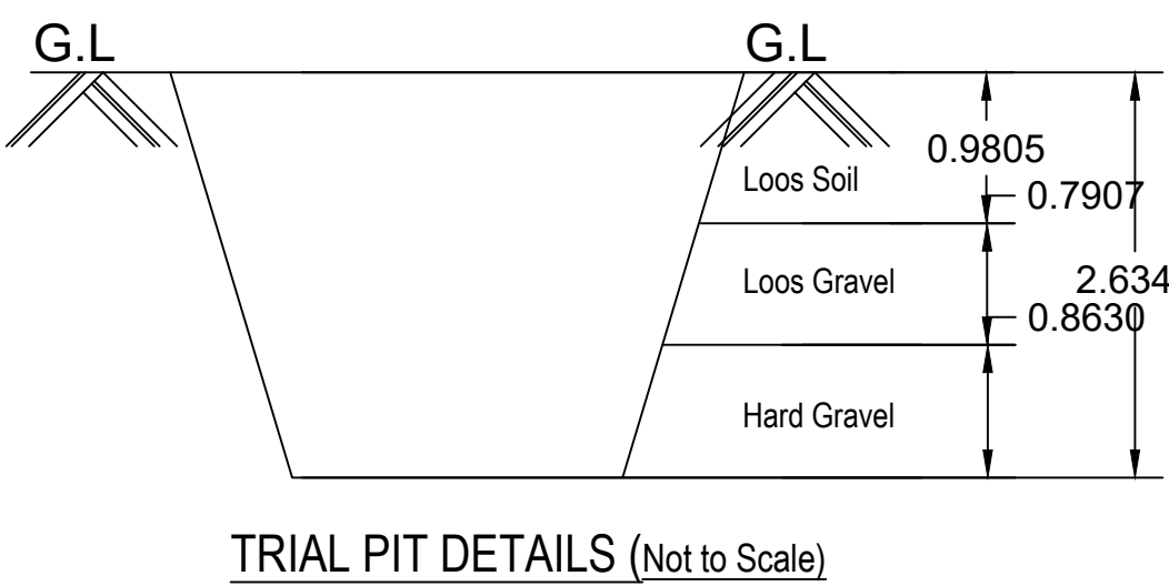
TRIAL PIT DETAILS (Not to Scale)
