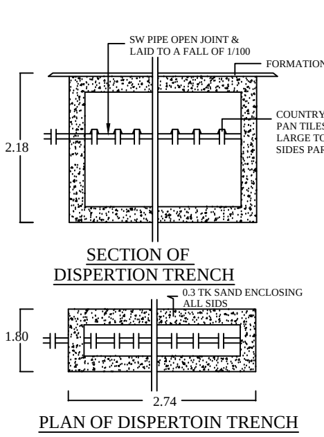
DISPERSION TRENCH
