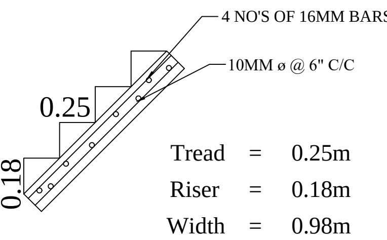
STAIRCASE DETAILS
