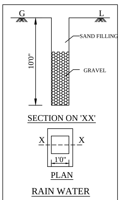
RAINWATER HARVESTING
