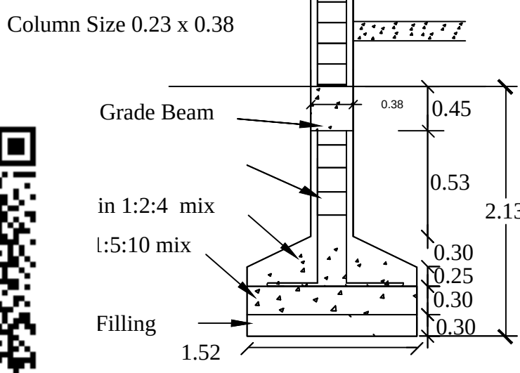
COLUMN DETAILS
