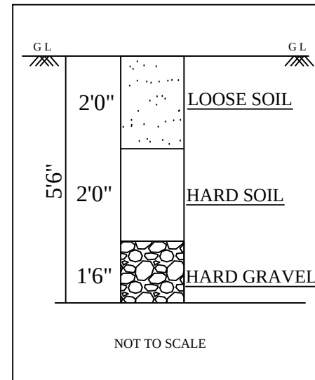
TRIAL PIT
