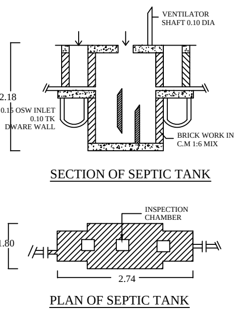
SEPTIC TANK
