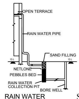
RAIN WATER
