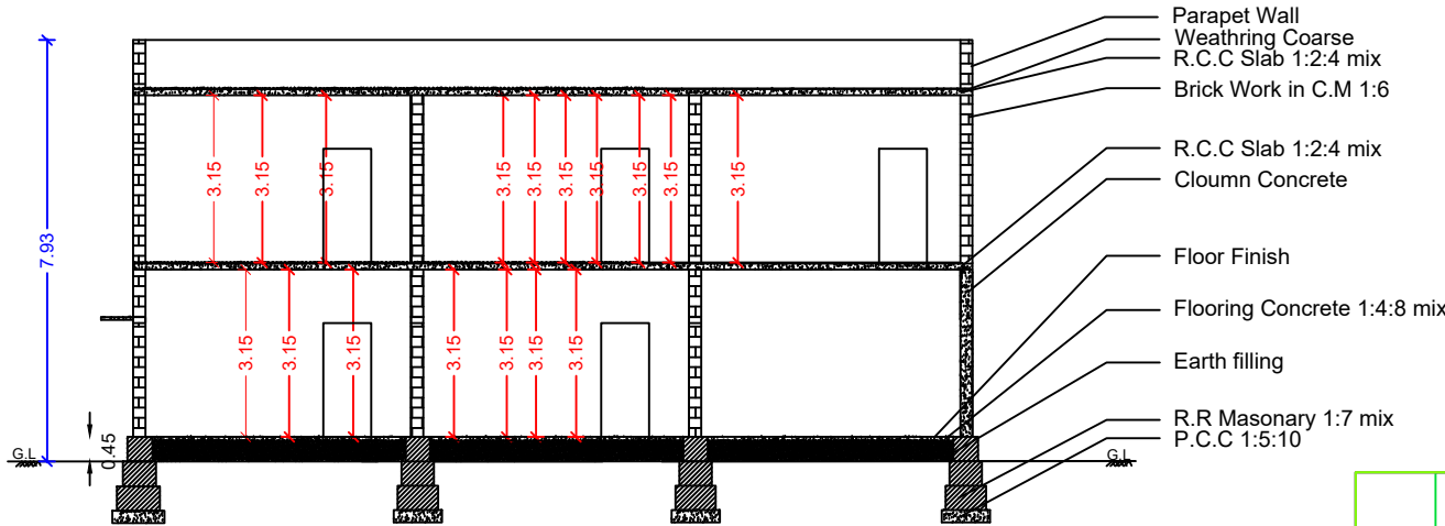
SECTION-AA
