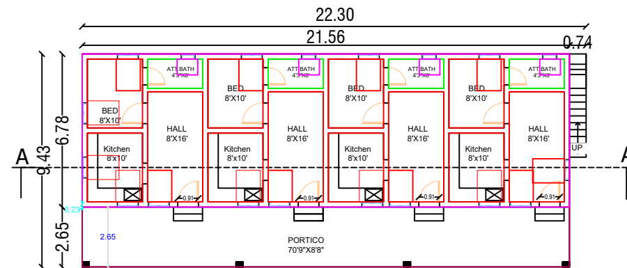
GROUND FLOOR PLAN FACING EAST
