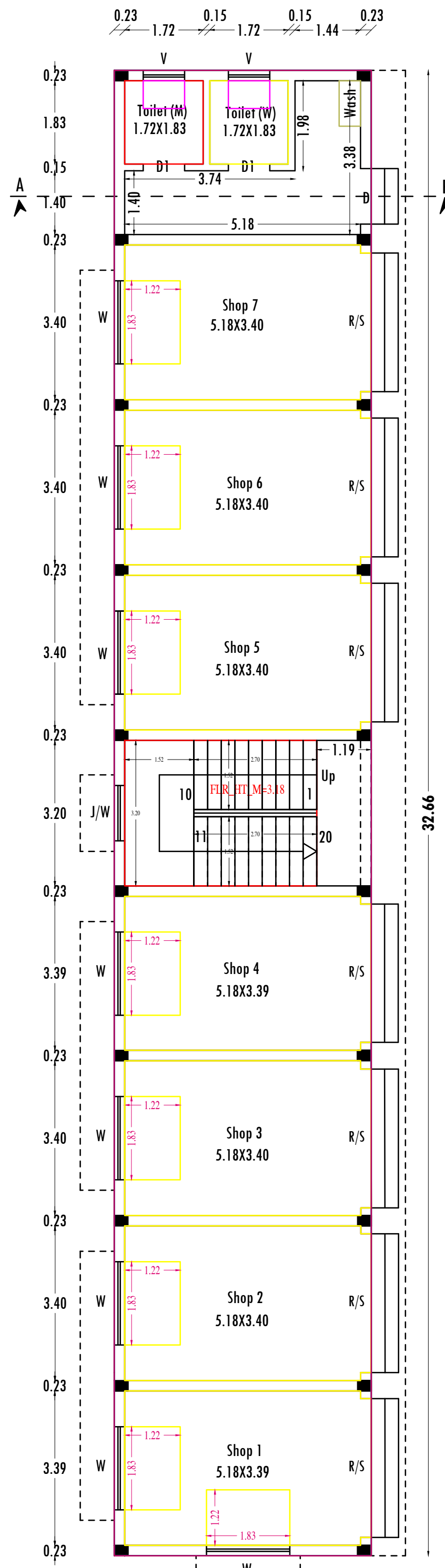
Ground Floor Scale:- 1:100
