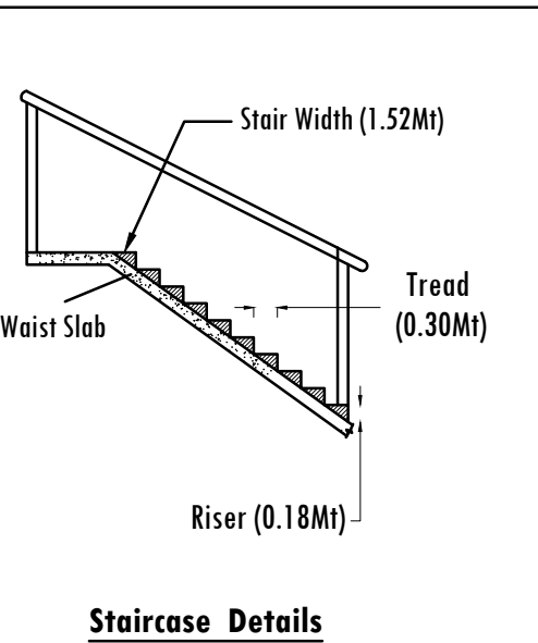
Staircase Details
