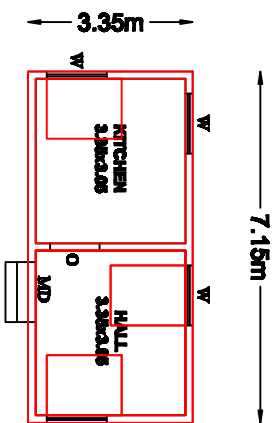
FLOOR - GROUND
