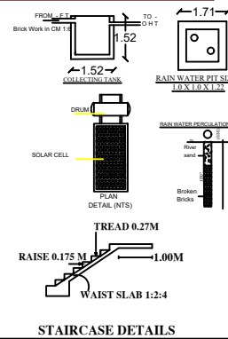
STAIRCASE DETAILS
