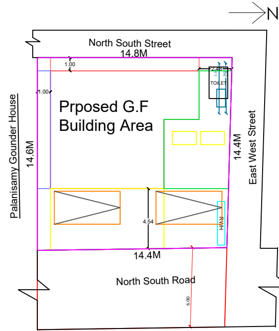
SITE PLAN
