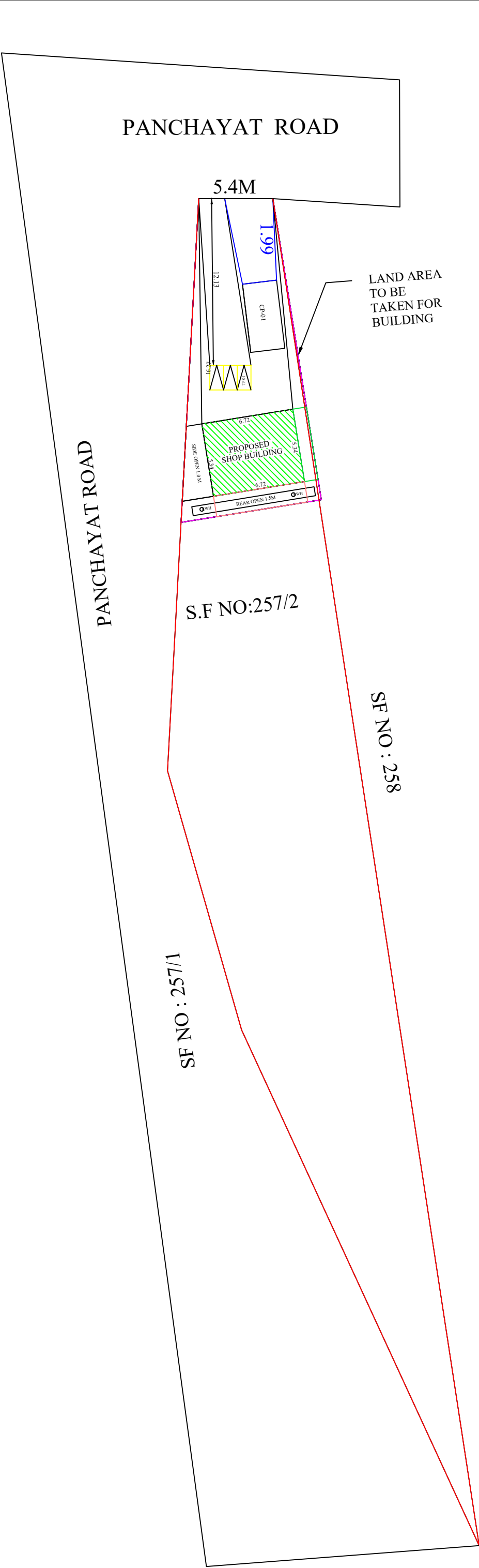
SITE PLAN-NOT TO SCALE
