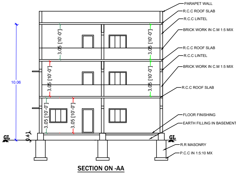
SECTION ON-AA
