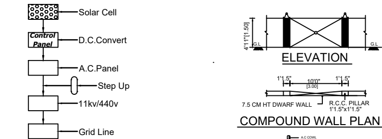
Solar System Flow Diagram
