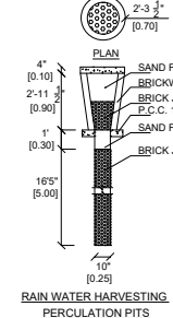
RAIN WATER HARVESTING PERCOLATION PITS
