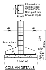
COLUMN DETAILS
