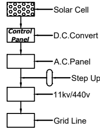
Solar System Flow Diagram
