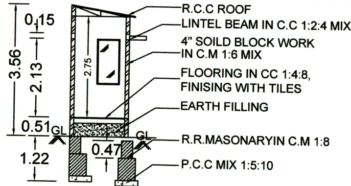
SECTION "A-B"
