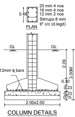
COLUMN DETAILS
