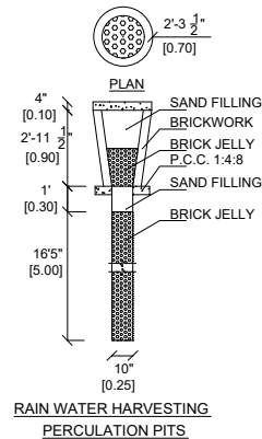
RAIN WATER HARVESTING PERCOLATION PITS
