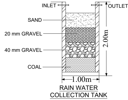
RAIN WATER COLLECTION TANK
