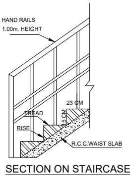
SECTION ON STAIRCASE
