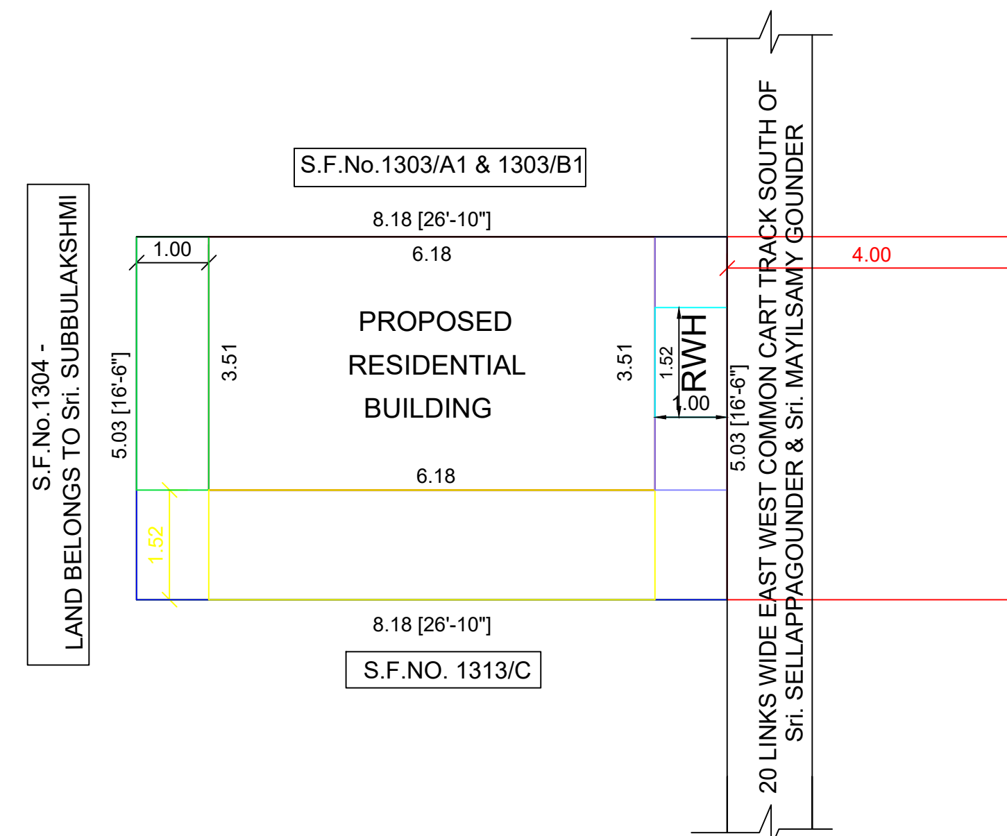
SITE PLAN
