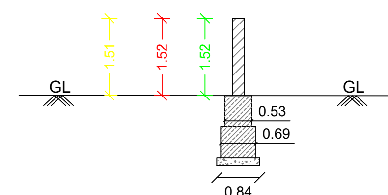
COMPOUND WALL
