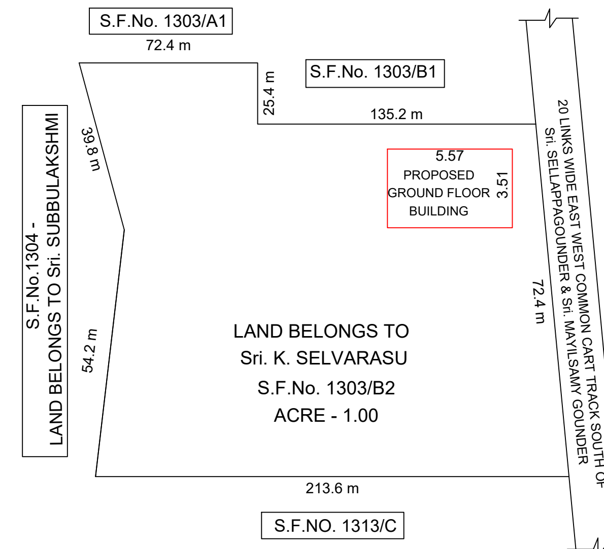
SITE PLAN - SCALE - NTS
