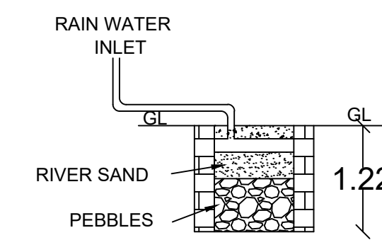
SECTIONAL ELEVATION
