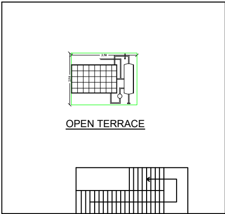
SITE PLAN:PROPOSED SCALE 1:100
