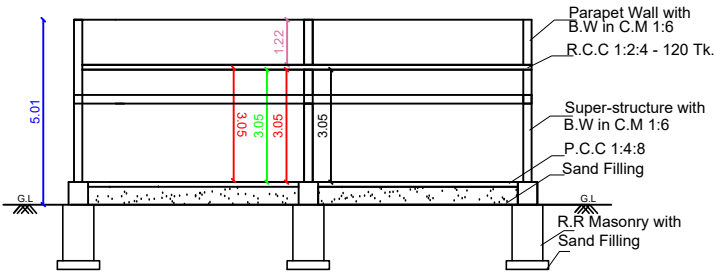
DETAILED PLAN: SCALE 1:100
