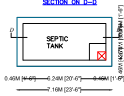
PLAN OF SEPTIC TANK SCALE 1"=2'-0"
