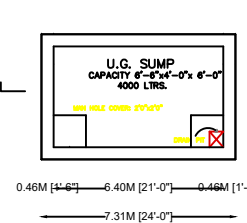
SUMP DETAIL SCALE 1"=4'-0"
