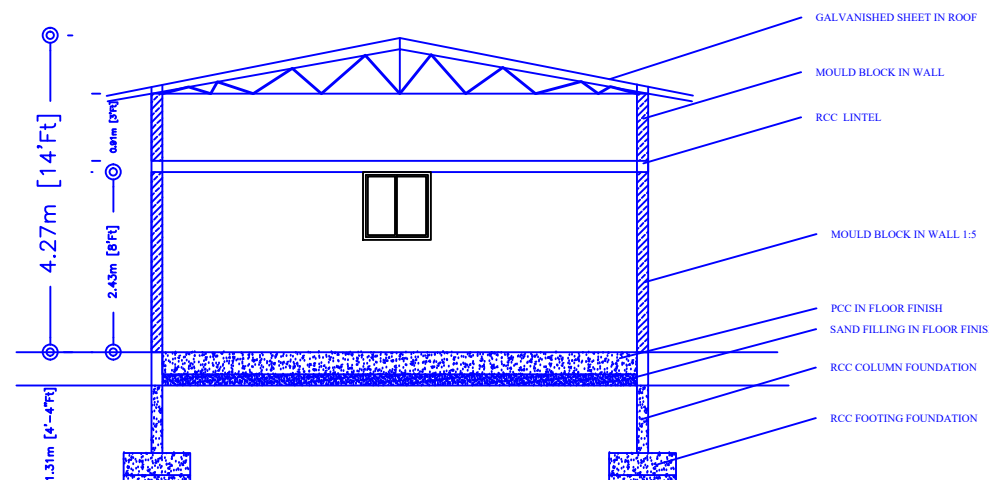
SECTION GODOWN - I
