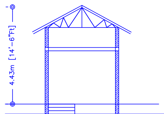
ELEVATION NORTH FACING LABOUR SHED - II
