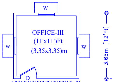
GROUND FLOOR PLAN OFFICE - III
