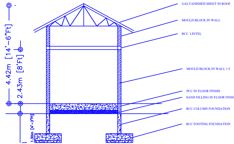
SECTION LABOUR SHED - II
