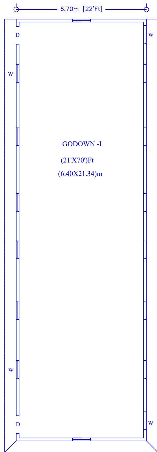
GROUND FLOOR PLAN GODOWN - I
