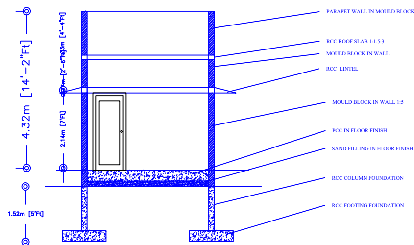
SECTION OFFICE - II
