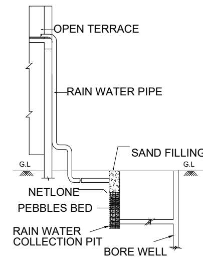
RAIN WATER
