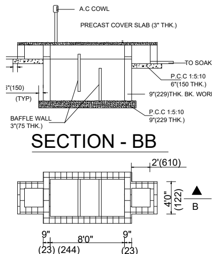
AN OF SEPTIC TANK
