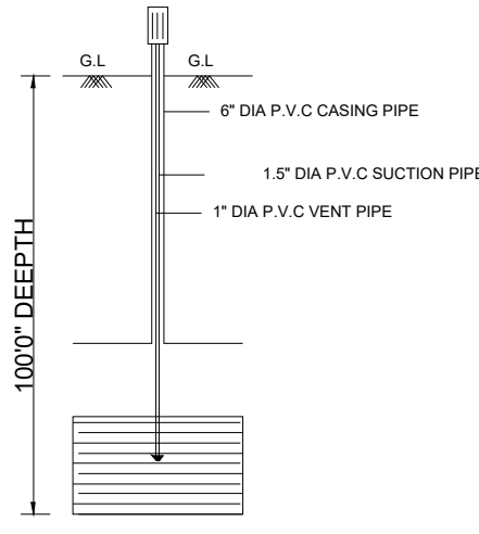
BORE WELL
