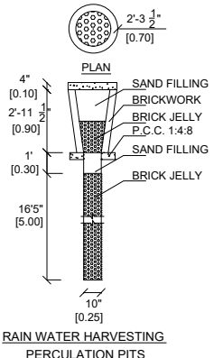
RAIN WATER HARVESTING PERCOLATION PITS
