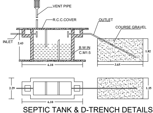
SEPTIC TANK & D-TRENCH DETAILS
