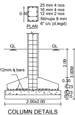
COLUMN DETAILS
