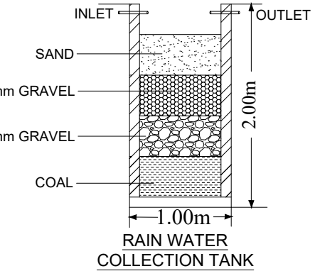
RAIN WATER COLLECTION TANK
