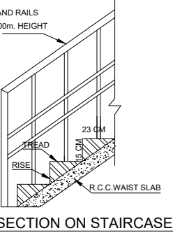
SECTION ON STAIRCASE
