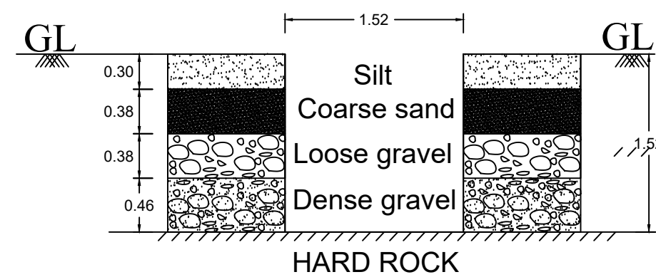
TRAIL PIT Not To Scale
