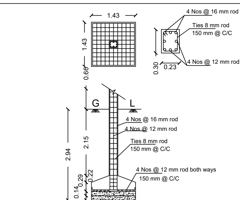
COLUMN AND FOOTING DETAILS
