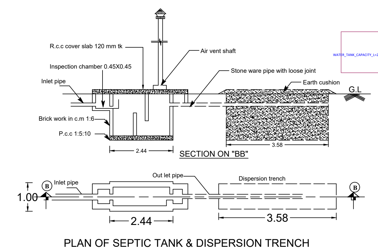
PLAN OF SEPTIC TANK & DISPERSION TRENCH
