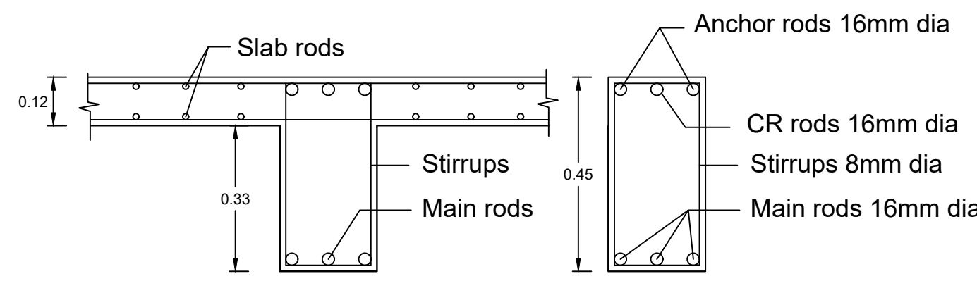
ROOF SLAB & BEAMS DETAILS (Not To Scale)
