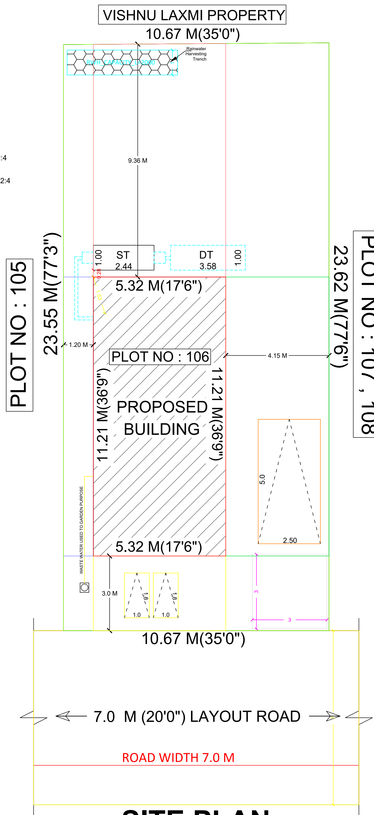
SITE PLAN
