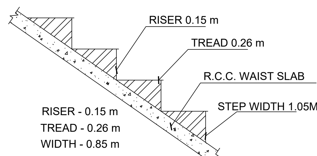
STAIRCASE DETAILS
