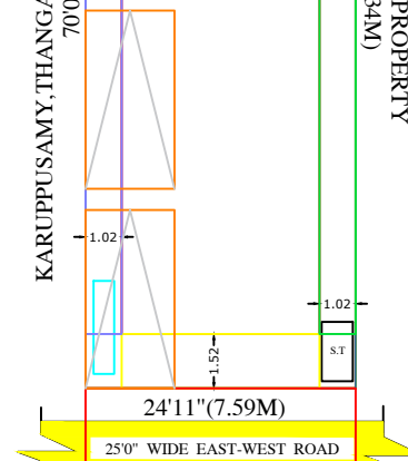
SITE PLAN
