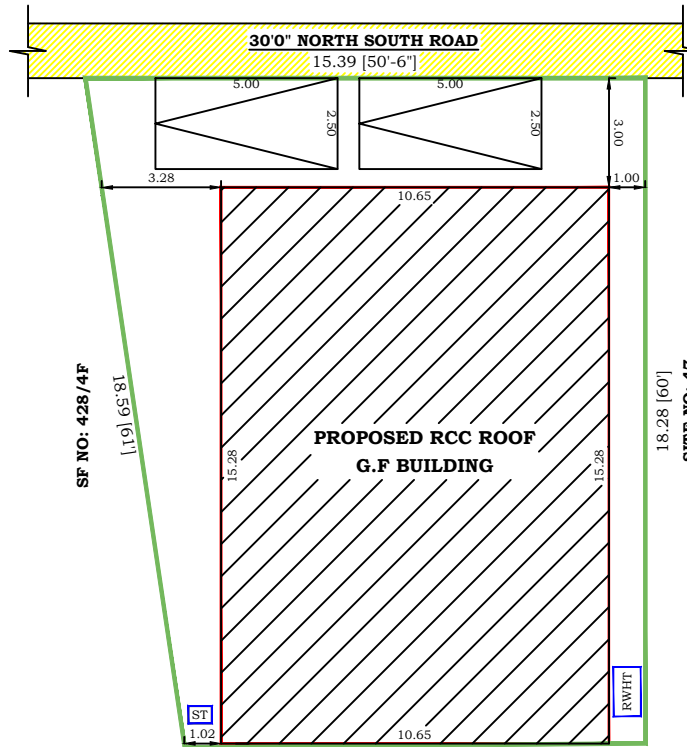
SITE NO: 45 SITE PLAN
