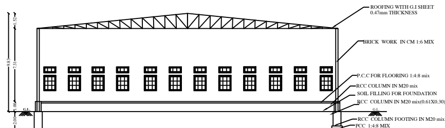
SECTION ON "AA" (BLOCK-1)
