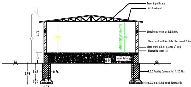
Section on "BC"
