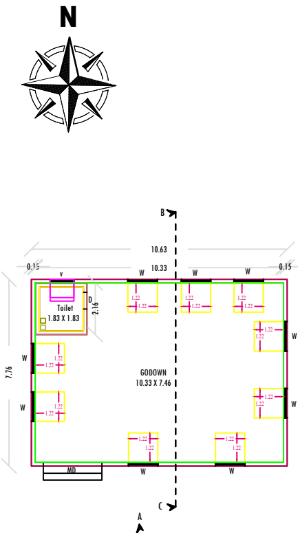
Floor-Ground Scale:- 1:100
