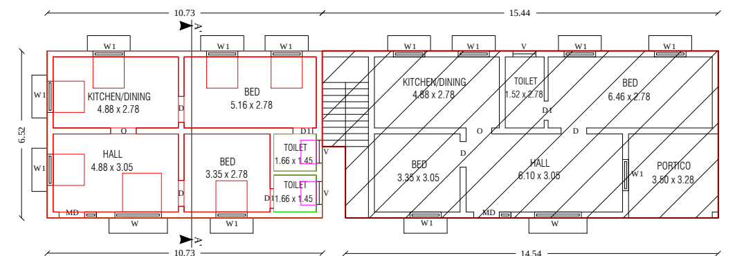
EXI & PRO.GROUND FLOOR PLAN
