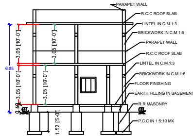
SECTION ON-AA
