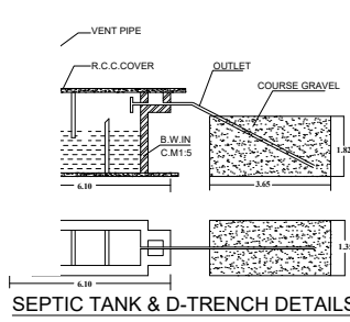
SEPTIC TANK & D-TRENCH DETAILS
