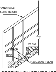
SECTION ON STAIRCASE
