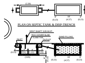
SECTION ON SEPTIC TANK & DISP-TRENCH
