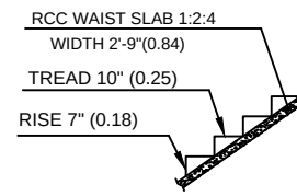
STAIRCASE DETAIL
