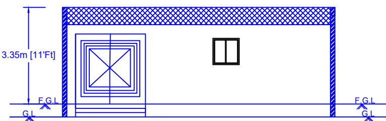
ELEVATION WEST FACING
