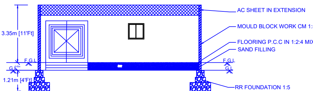
SECTION ON-AA
