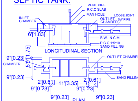
SEPTIC TANK:
