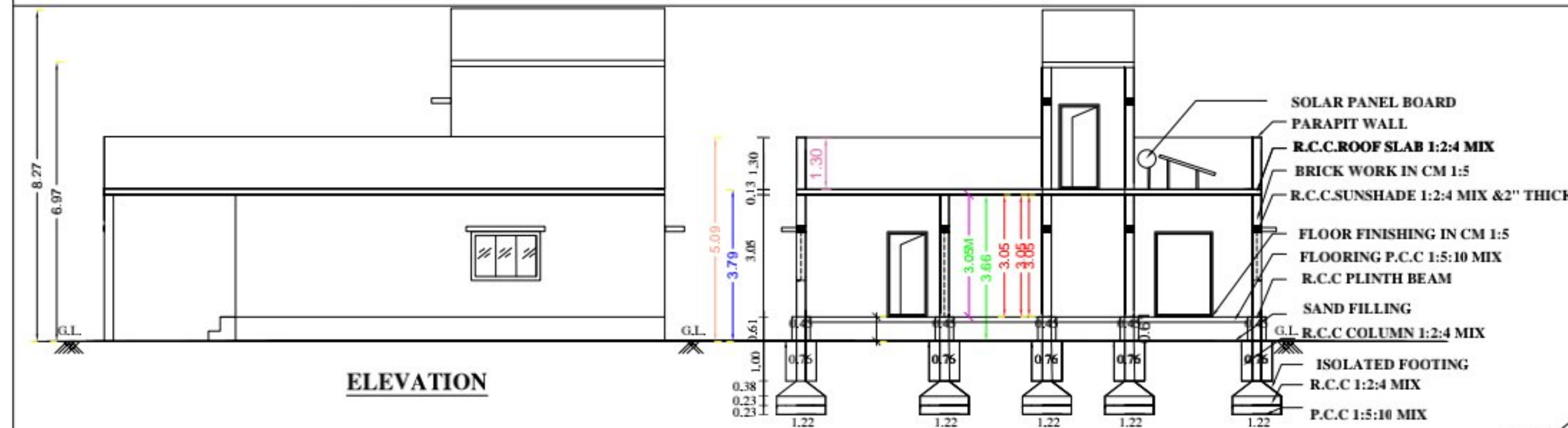
SECTION ON AA SITE NO: 86 PART , 87 , 88 PART
